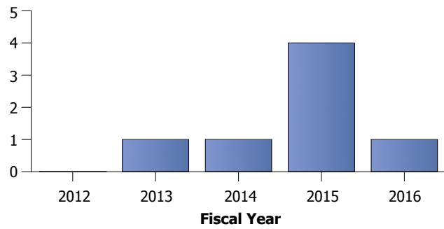
Burglary
